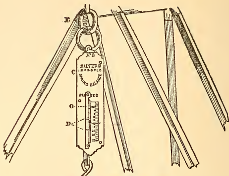
FIG. 10. CROOKES' APPARATUS.
