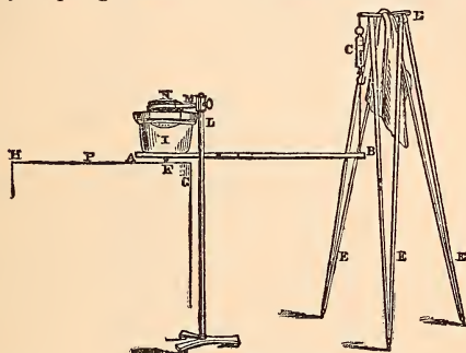
FIG. 9. CROOKES' APPARATUS.
