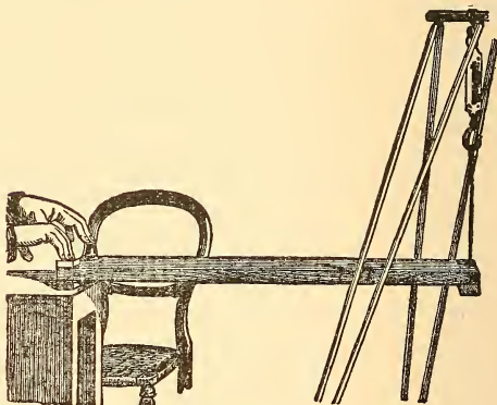
FIG. 8. CROOKES' APPARATUS.
