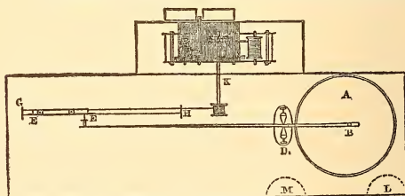
FIG. 16. SECOND CROOKES' APPARATUS.
