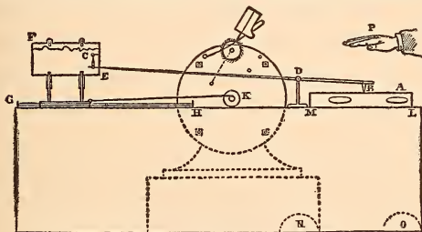
FIG. 17. SECTION OF APPARATUS IN FIG. 16.
