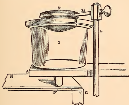
FIG. II. CROOKES' APPARATUS.
