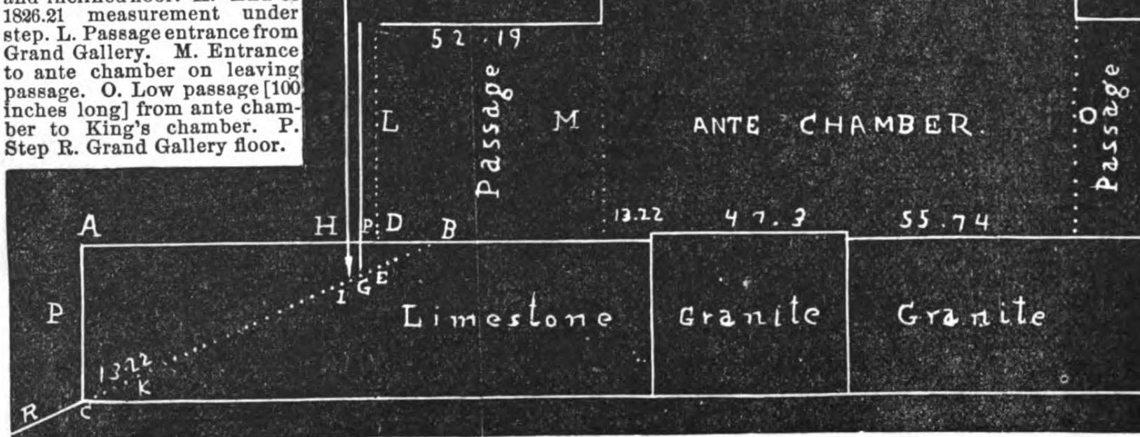
Vertical Longitudinal Section of the Floor of the Step, Passage and Ante-Chamber.
