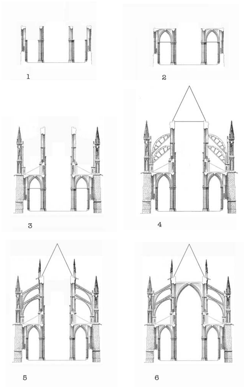
The sequence of cathedral construction according to John Fitchen.
