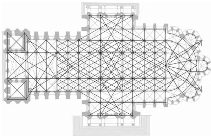
The geometrical scheme underlying the design of Chartres, as proposed by historian Nigel Hiscock.
