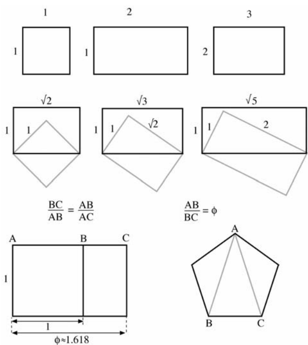
Some common ratios in medieval church architecture, and how they are constructed. The lower two figures show the Golden Mean \phi and how it is related to the proportions of a pentagon.
