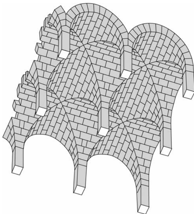
The groin vault.
