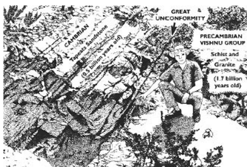
Frenchman Mountain "Great Unconformity" where the Vishnu schist and granite were tilted about 50 degrees to the east some ten million years ago during the Miocene Epoch. Graphic by University of Los Vegas Geoscience Department.
