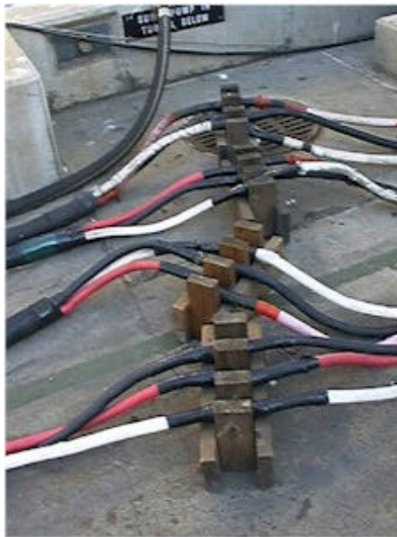
Figure 12-10 A 480-volt shore-cable to ship-cable splice connection in place
