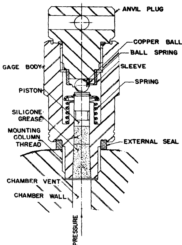
EXTERNAL CRUSHER GAGE T14 (US)
