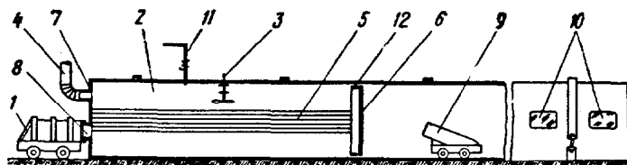
RUSSIAN TESTING GALLERY, MAKNII, AND ACCESSORIES
