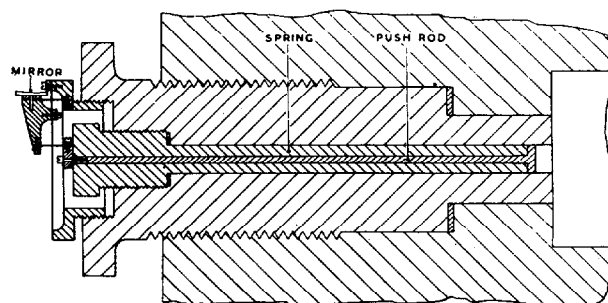
ARE SPRING GAUGE, SECOND DESIGN
