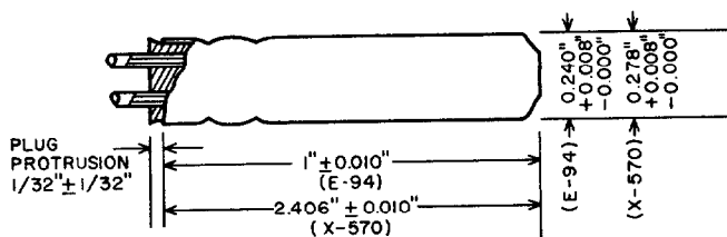
Special DuPont Blasting Caps E94 1" × 0.240" and X-570 2.406 × 0.278"
