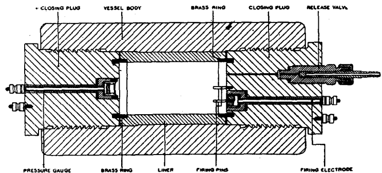
BRITISH CLOSED VESSEL
