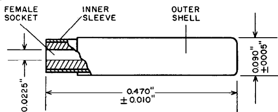
Special DuPont Blasting Cap X-549C 0.470" × 0.090" Plug-in Type
