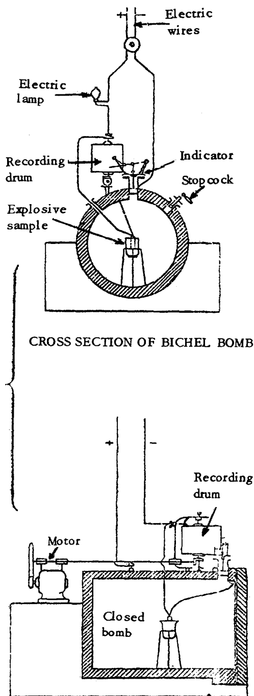
SIDE VIEW OF BICHEL BOMB
