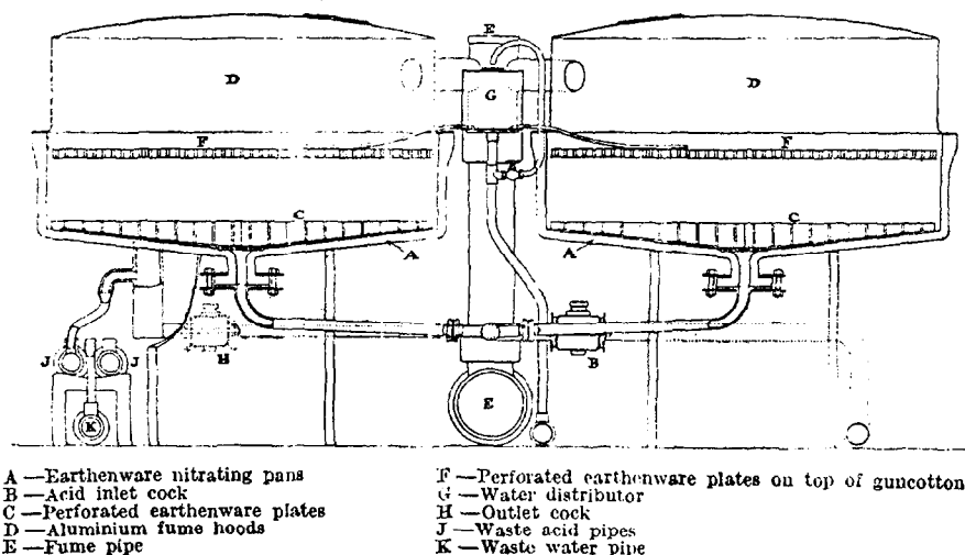
WALTHAM ABBEY GUNCOTTON DISPLACEMENT PLANT
