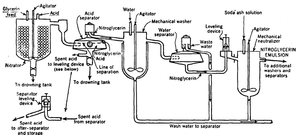
BLIAZZI CONTINUOUS METHOD FOR MANUFACTURING NG
