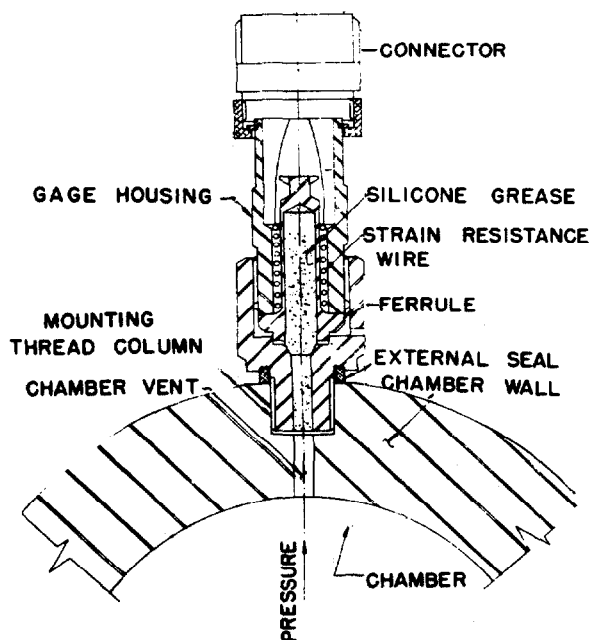
CROSS SECTION OF STRAIN RESISTANCE WIRE TRANSDUCER PRESSURE GAGE, MODEL C-AN
