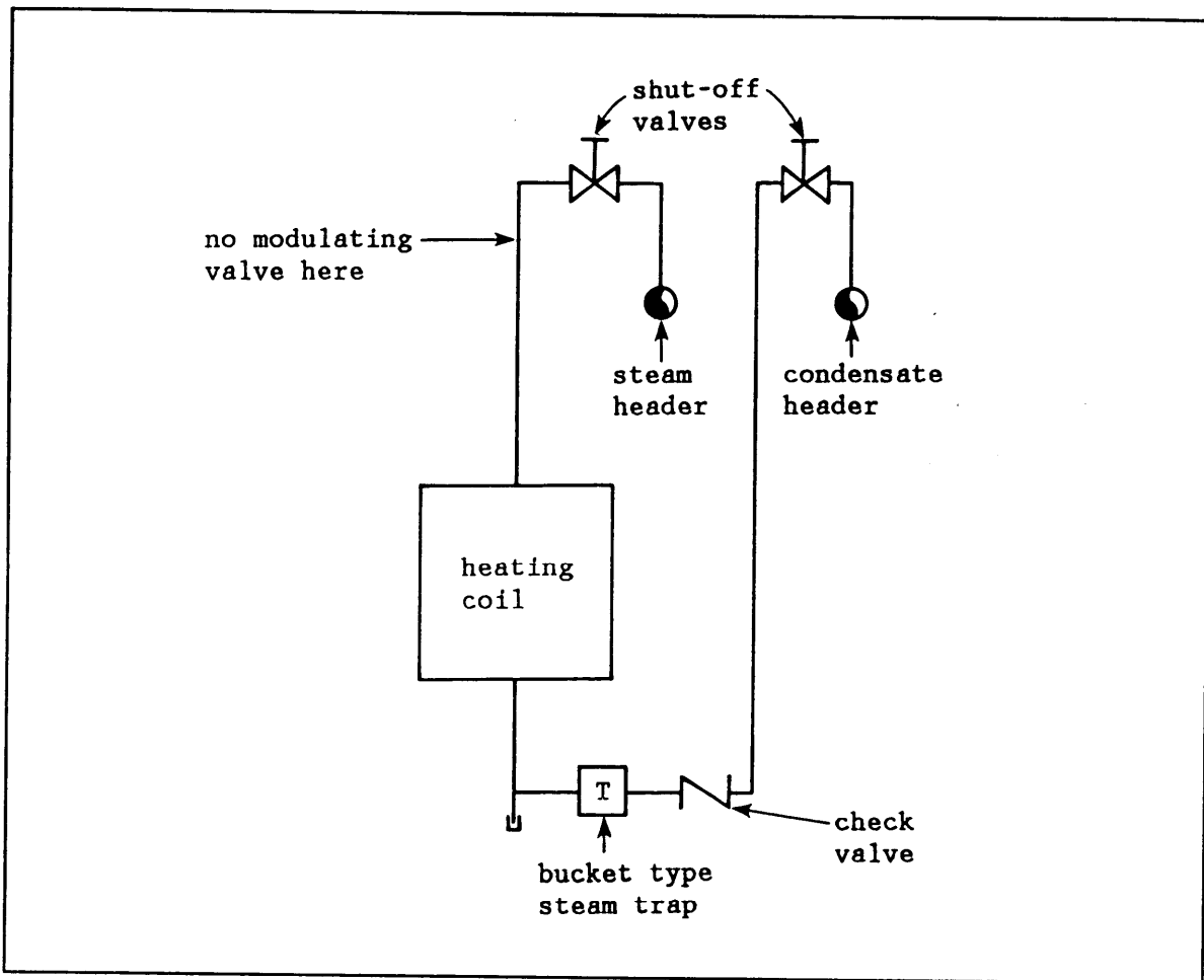
Figure 92 Lifting Condensate to an Overhead Return Header
