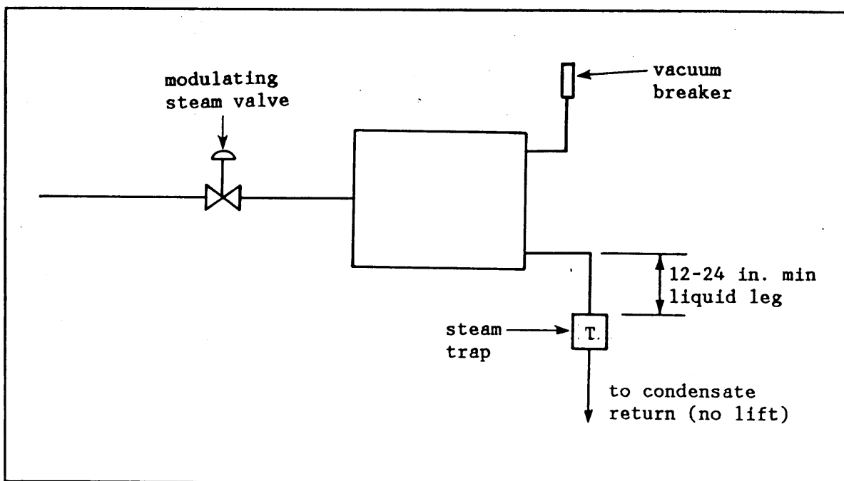
Figure 93 Modulated Steam Coil With Vacuum Breaker and 12- to 24-Inch Minimum Liquid Leg
