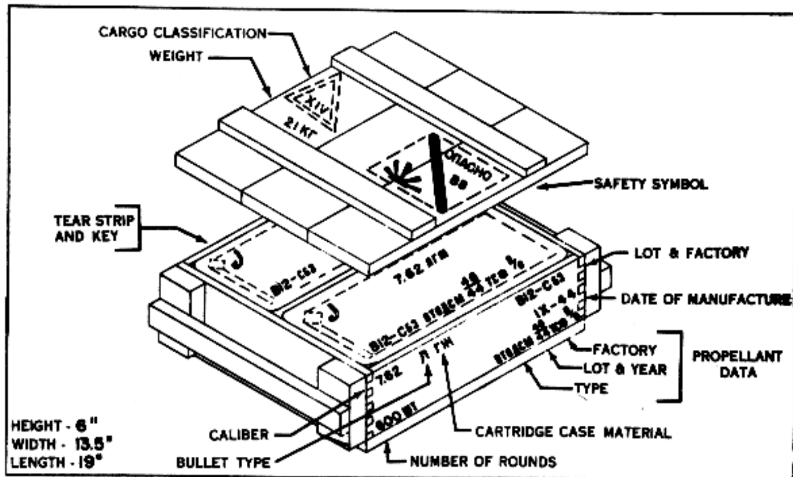
FIGURE 35. SOVIET AMMUNITION BOX.
