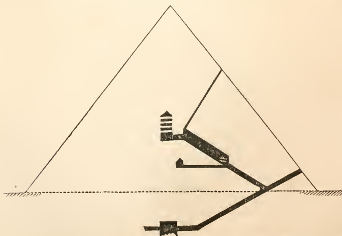
FIG. 14. SECTION OF THE GREAT PYRAMID OF GIZEH, EGYPT.
