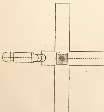
FIG. 9. PLAN OF SEPULCHRAL CHAMBER AT MITLAN.
