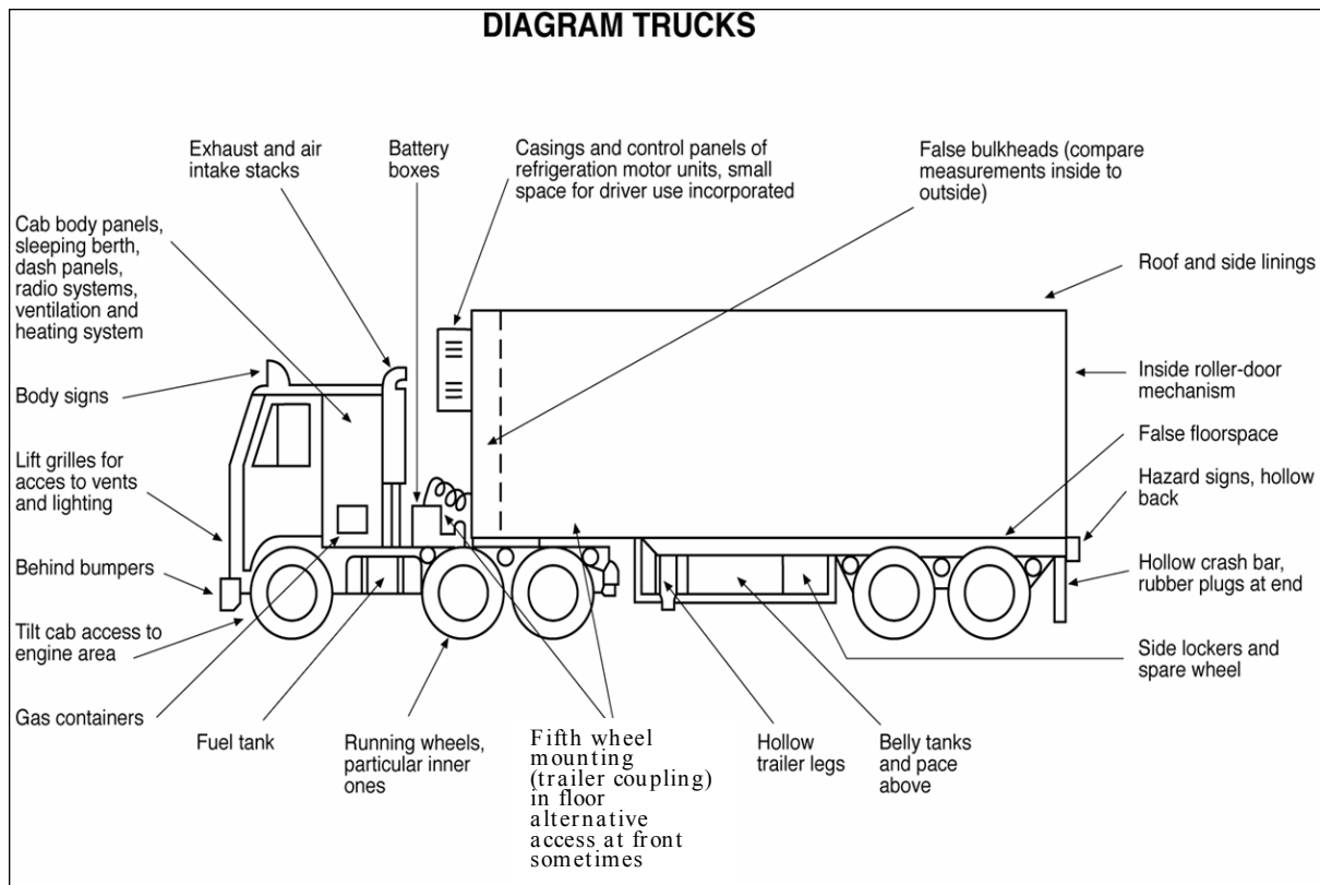
Figure IV-5 Truck Diagram
