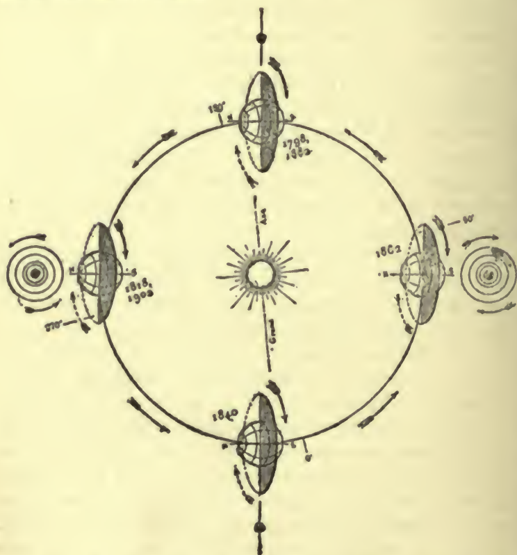
Fig. 1.—The inclination of the system of Uranus. Aspects seen from the earth at the four extreme positions.
