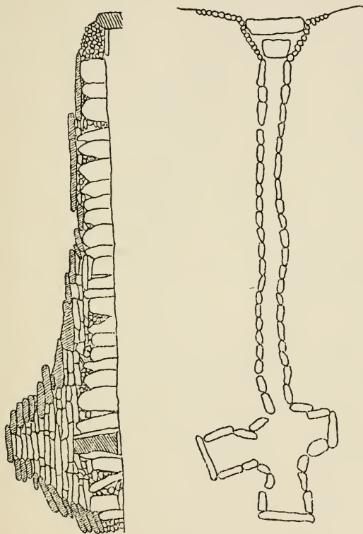
FIG. 8. Corridor-tomb at New Grange, Ireland. (Coffey, Transactions of the Royal Irish Academy , 1892.)
