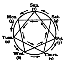
FIG. 7.—Heptacle on which the 7-square is based.
