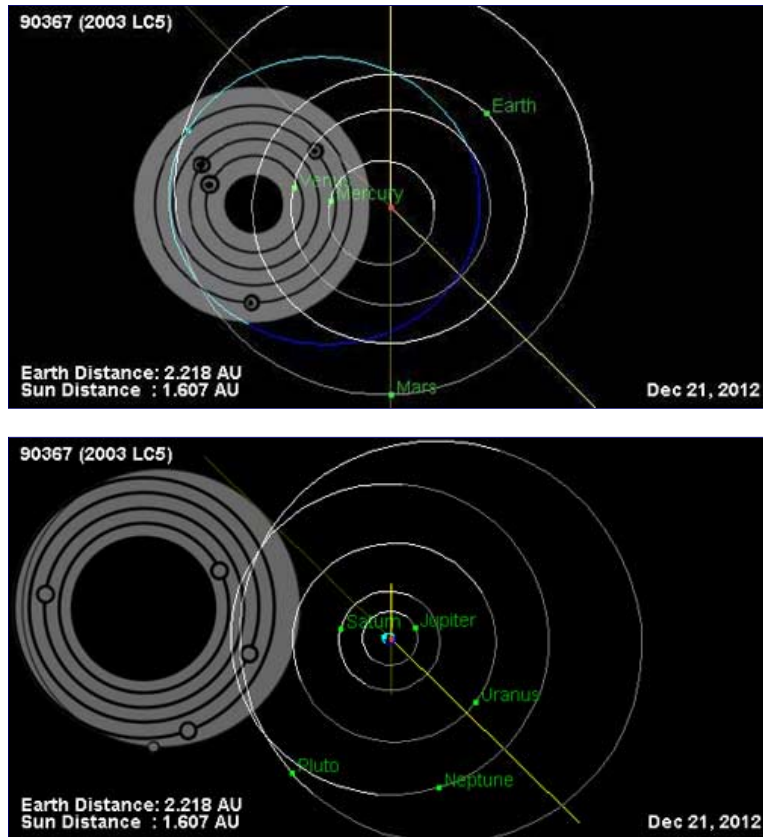
Earthfiles viewer submitted projected planetary positions in our solar system on December 21, 2012.
