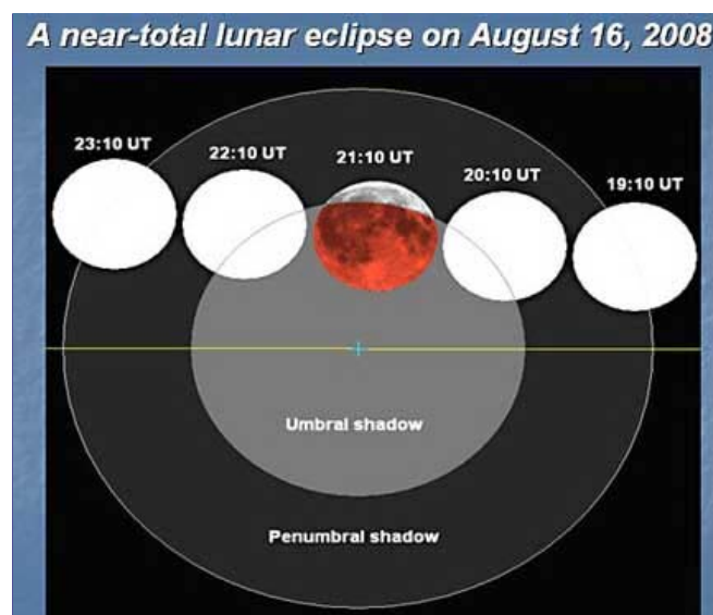
Partial lunar eclipse on August 16, 2008. Graphic by NASA Eclipse Website .
