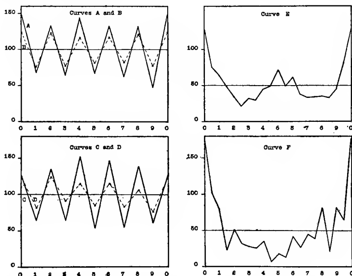
Plate XL.—Curves showing the Dependence of the ' équation décimale ' upon calibration-marks, and its independence of fractionation of decimal estimates.
