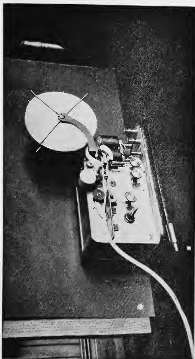
Fig. 16.— The Self-Recording Telegraph Instrument. ( Ibid. , p. 528.) (Size .25 diameters.)
