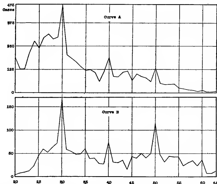
Plate XXIII.—Kymograph Time-Records. Curves of the frequency of estimates 2.0 to 6.3 units.
