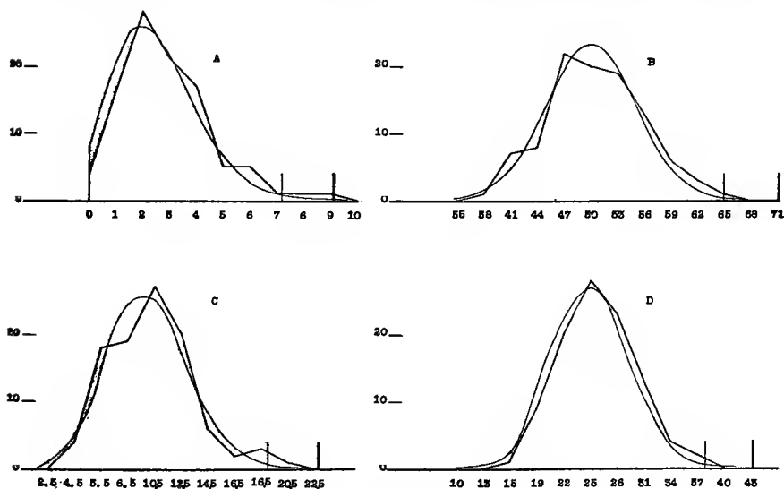
Plate XLII.—Distributions of R Cases in Card-Guessing. Sets of 100. 100 Reagents.
