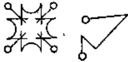
The Sun
