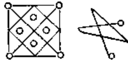
Mercury
