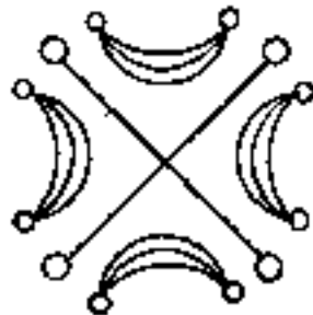
The Moon.
