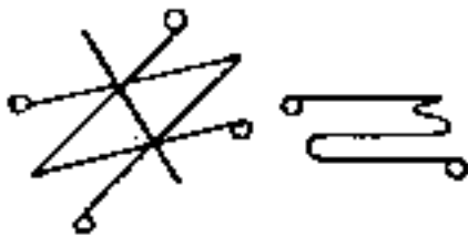
Saturn
