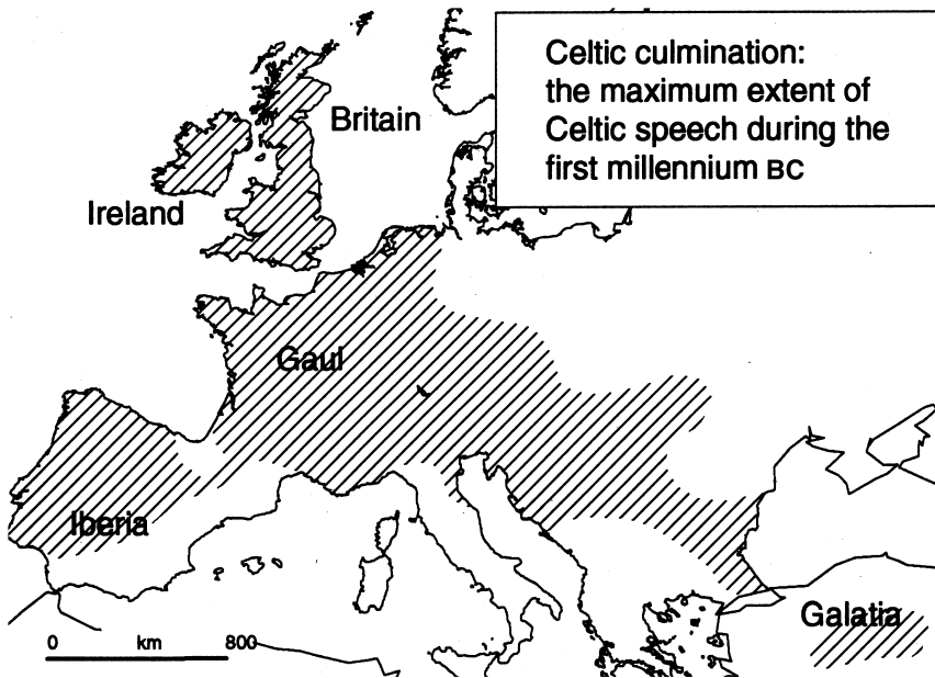
Figure 14.2 Culmination: a large part of Europe was at some time 'Celtic' according to most authorities, though the outline is variable in extent
