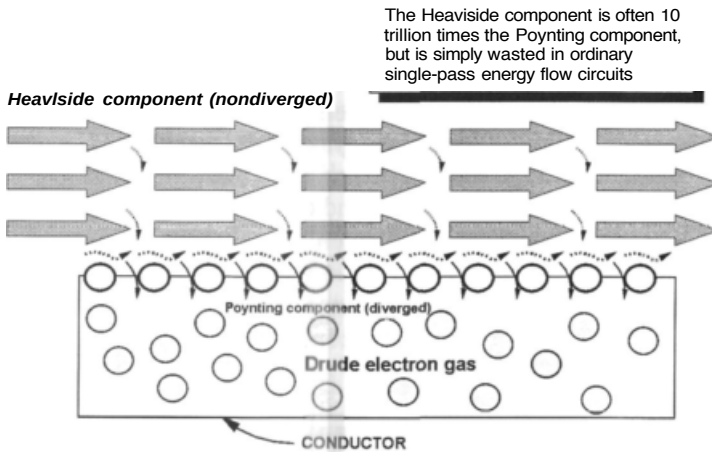
Figure 2-4 Heaviside nondivergent and Poynting divergent energy flow components.
