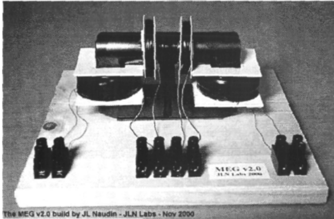
Figure 7.2 Naudin's Mark II Replication of the MEG.
