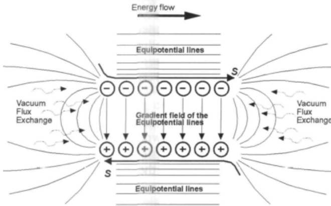
Figure 2-9 Paired conductors as an extended set of dipoles.
