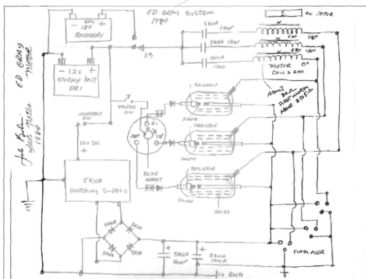
Figure 5-19 Page 2 from Bedini's lab notebook on the Gray conversion tube.
