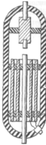
Figure 5-1S Gray's conversion tube used with power systems,
