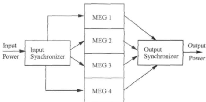
Figure 7-3 Block diagram of envisioned modular MEG design.
