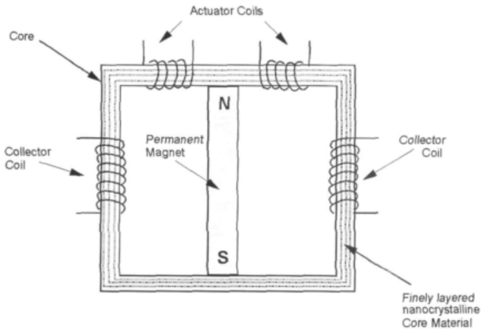
Figure 7-5 Diagrammatic drawing of the MEG.
