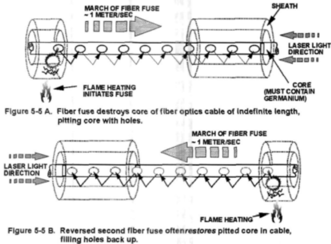
Figure 5-5 The fiber fuse.
